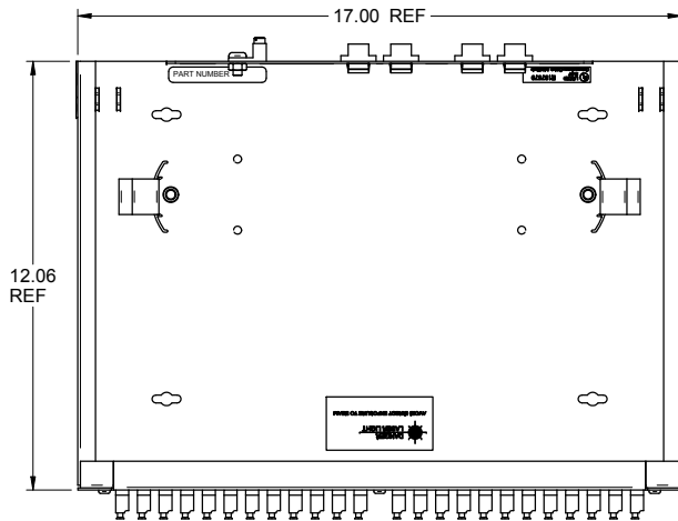
TOP VIEW (SHOWN WITHOUT COVER)
