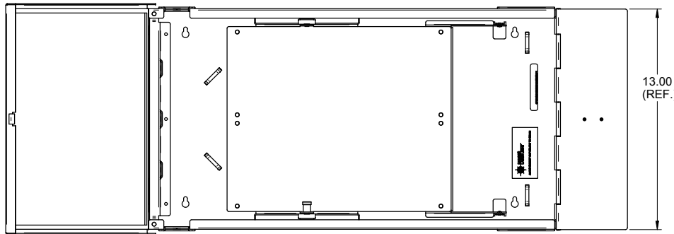
OCC P/N PROWTC-2ISM TOP VIEW (FRONT DOOR OPEN)
