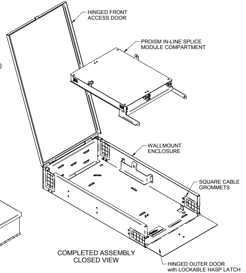
RIGHT SIDE (OUTER DOOR OPEN)
