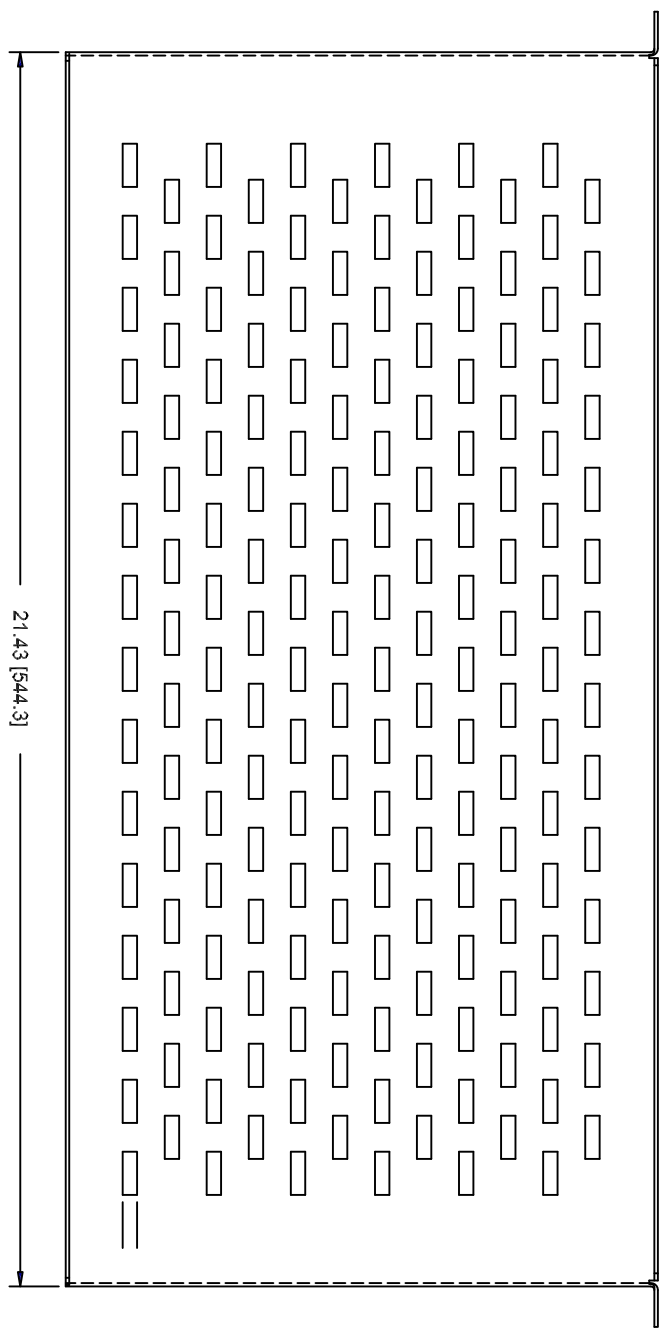
TOP VIEW
